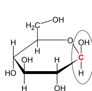
\beta -D-Glukosa
